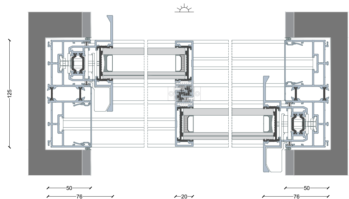
GAMME BAILUX 36 (double vitrage)
